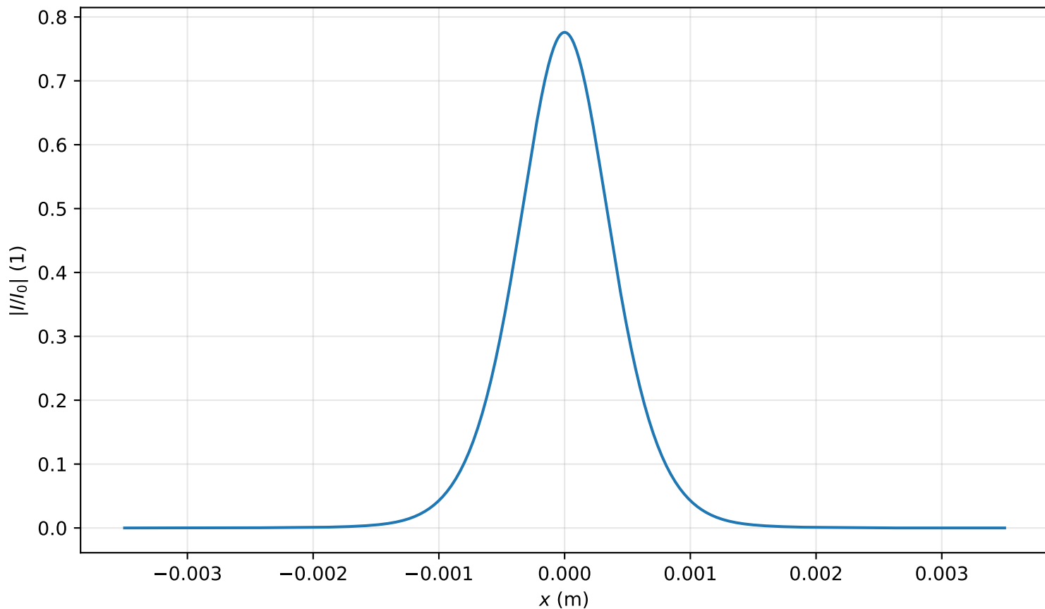
Intensity profile I(x, y = 0, z = 3.264m)/I_0 , P_{in}=0.7P_{cr} , artificial time
